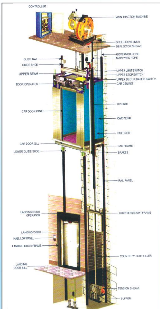
ELEVATOR MODEL
